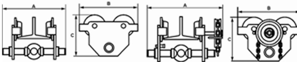
PLAIN TROLLEY
